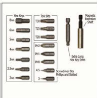
Screw Bits
